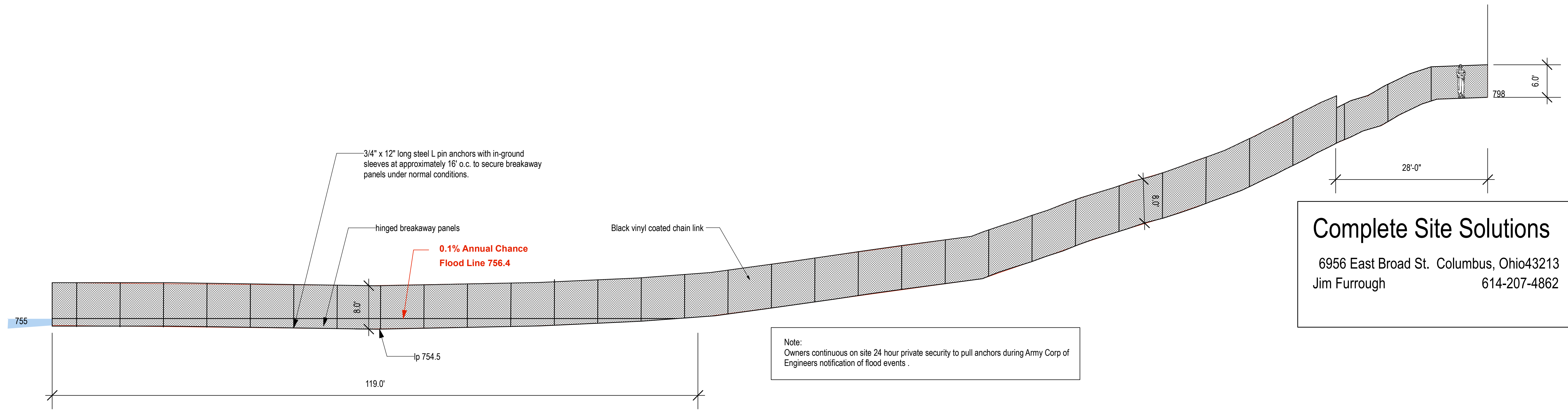
Fencing Plan Scale: 1" = 20'-0"
