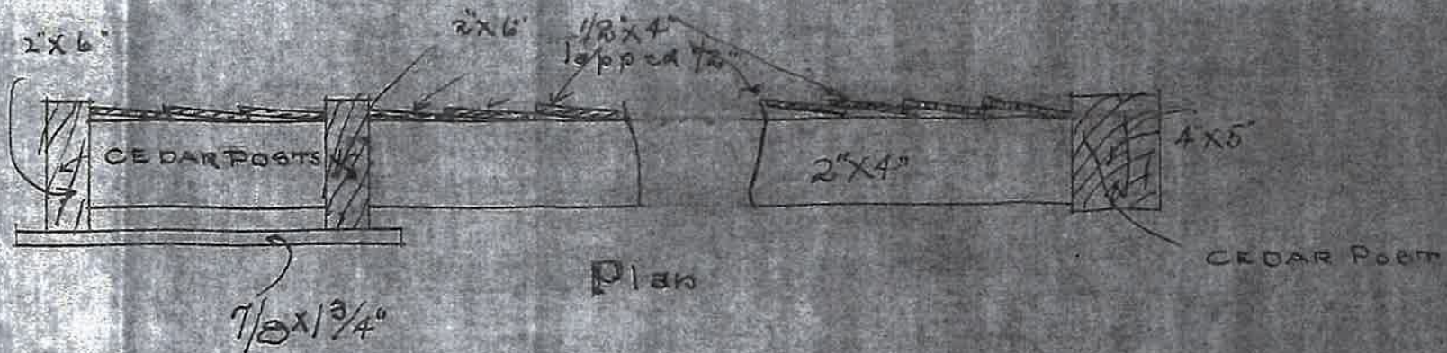
DETAIL of FENCE Scale 1/2" = 1 ft
