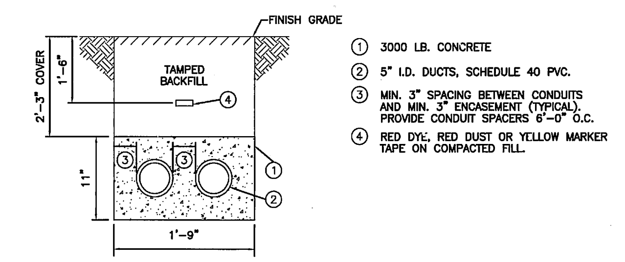
UNDERGROUND DUCTS SCALE: NONE B U100
