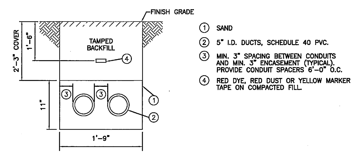
UNDERGROUND DUCTS SCALE: NONE A U100
