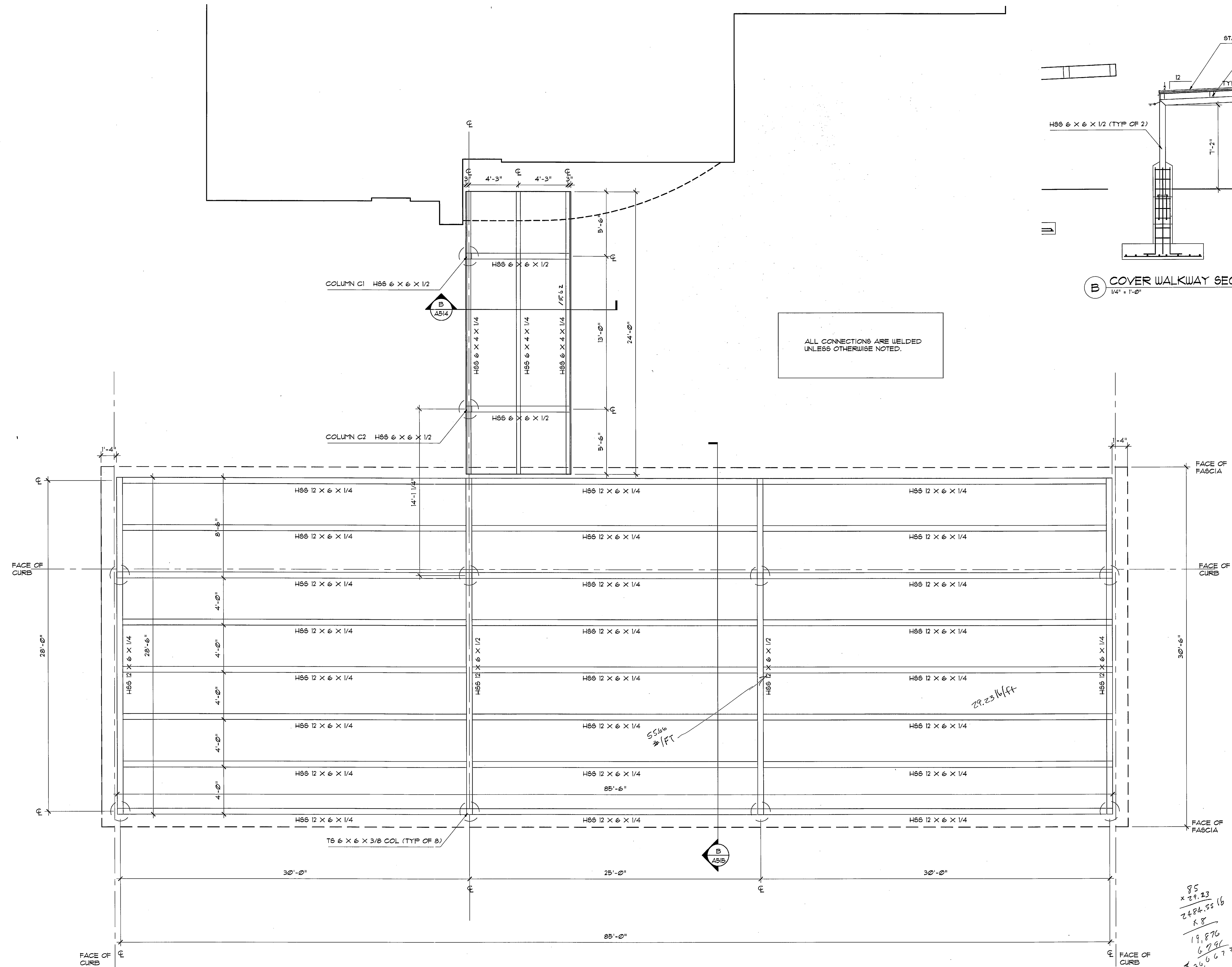
A CRUISER SHELTER PLAN 1/4" = 1'-0"
