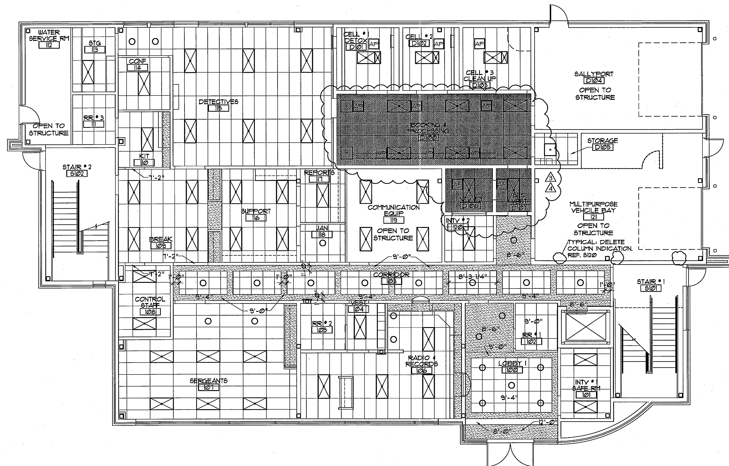
N FIRST FLOOR REFLECTED CEILING PLAN 1/8" = 1'-0"
