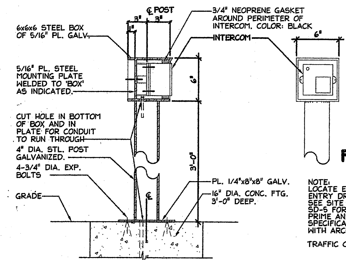
E INTERCOM POST SECTION 1/8" = 1'-0"
