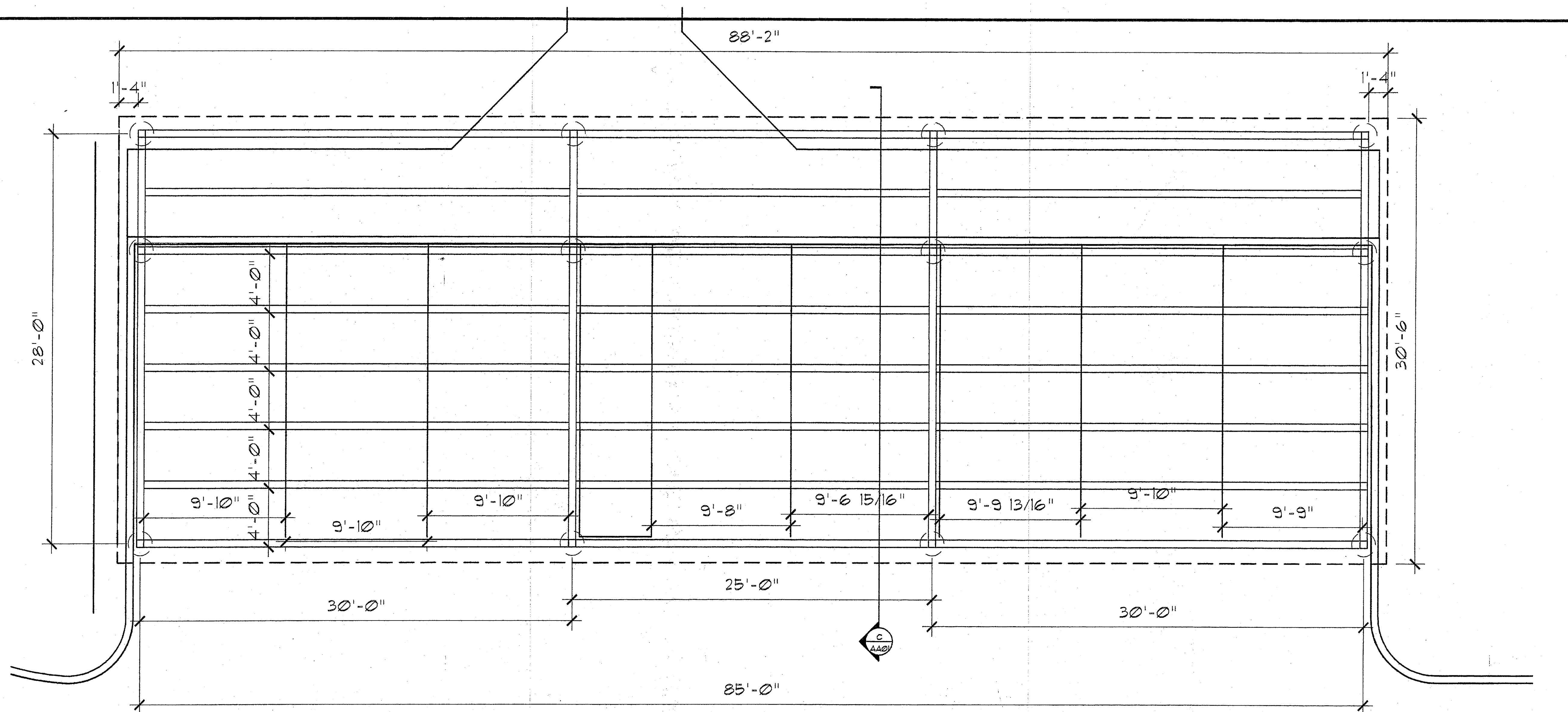
A CRUISER SHELTER PLAN 1/8" = 1'-0"
