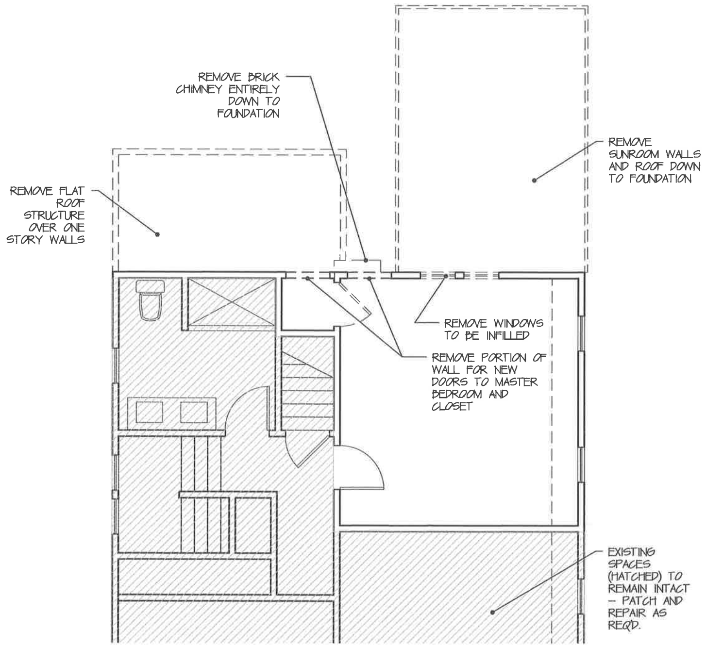
EXISTING/DEMO
