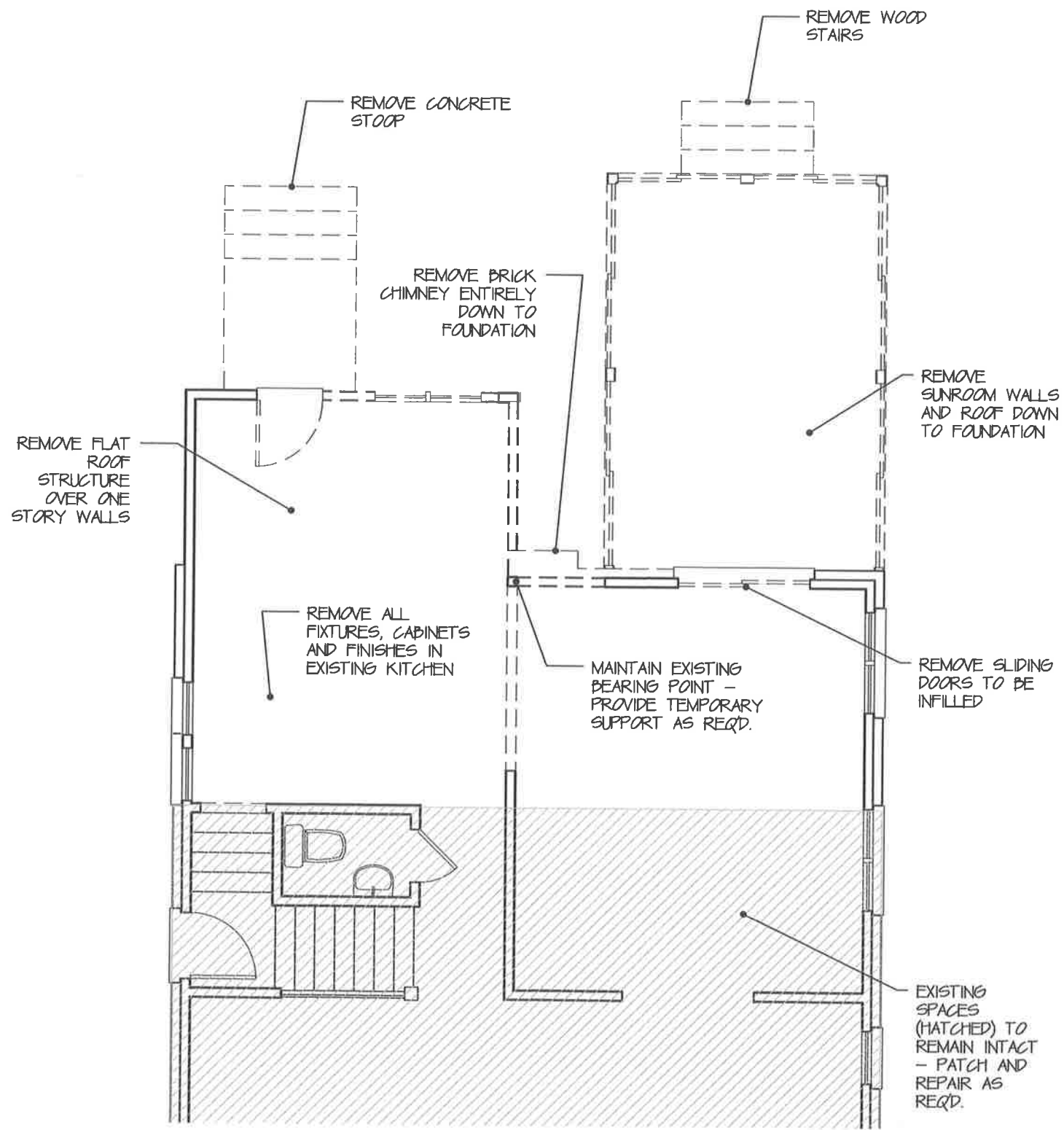
EXISTING/DEMO
