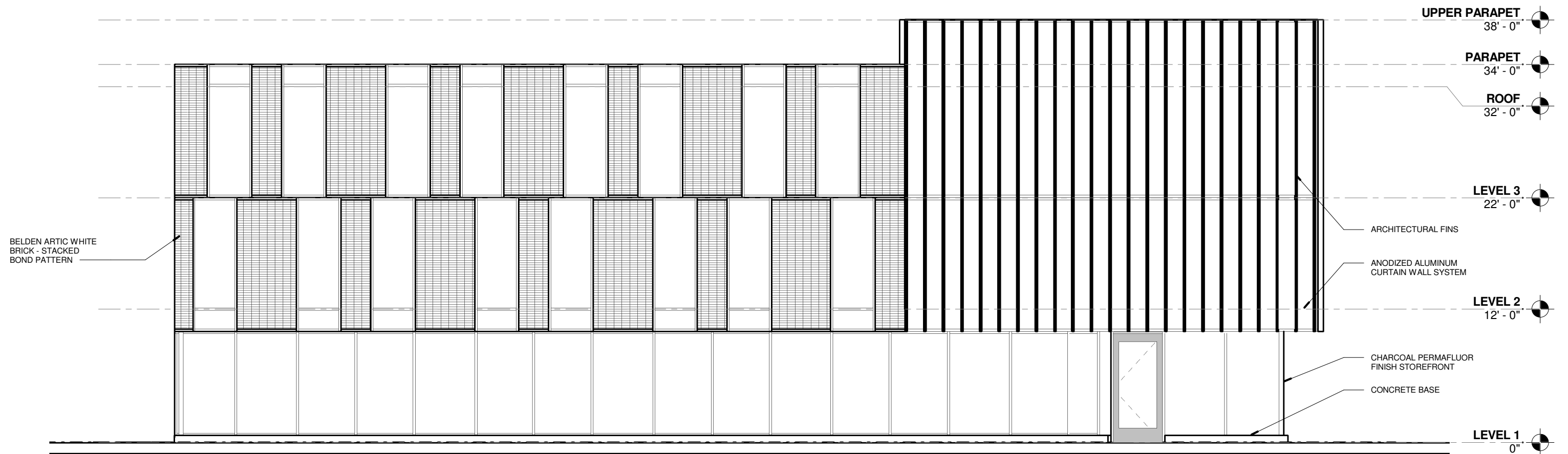
South Elevation
