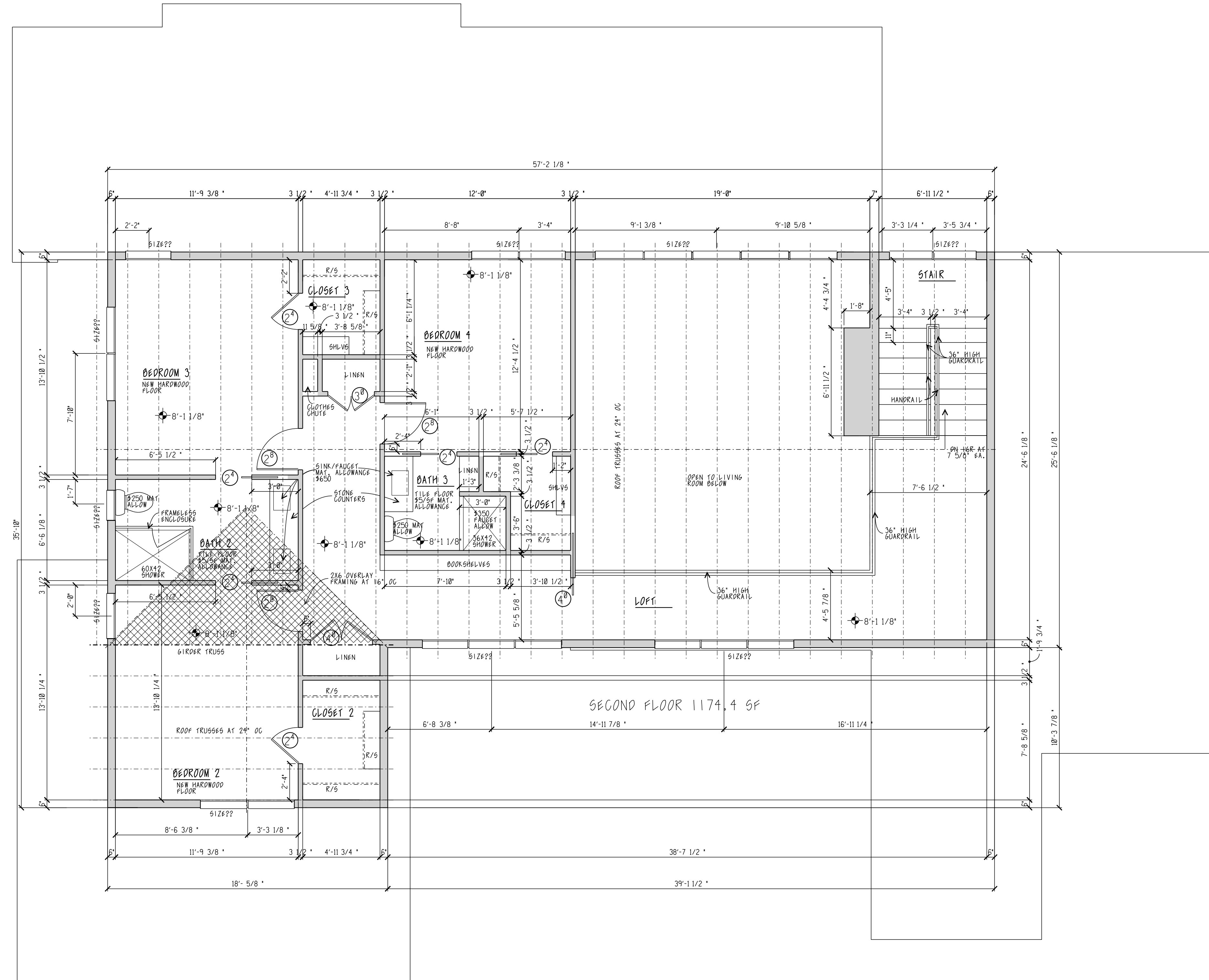
PROPOSED SECOND FLOOR PLAN SCALE: 1/4" = 1'-0"
