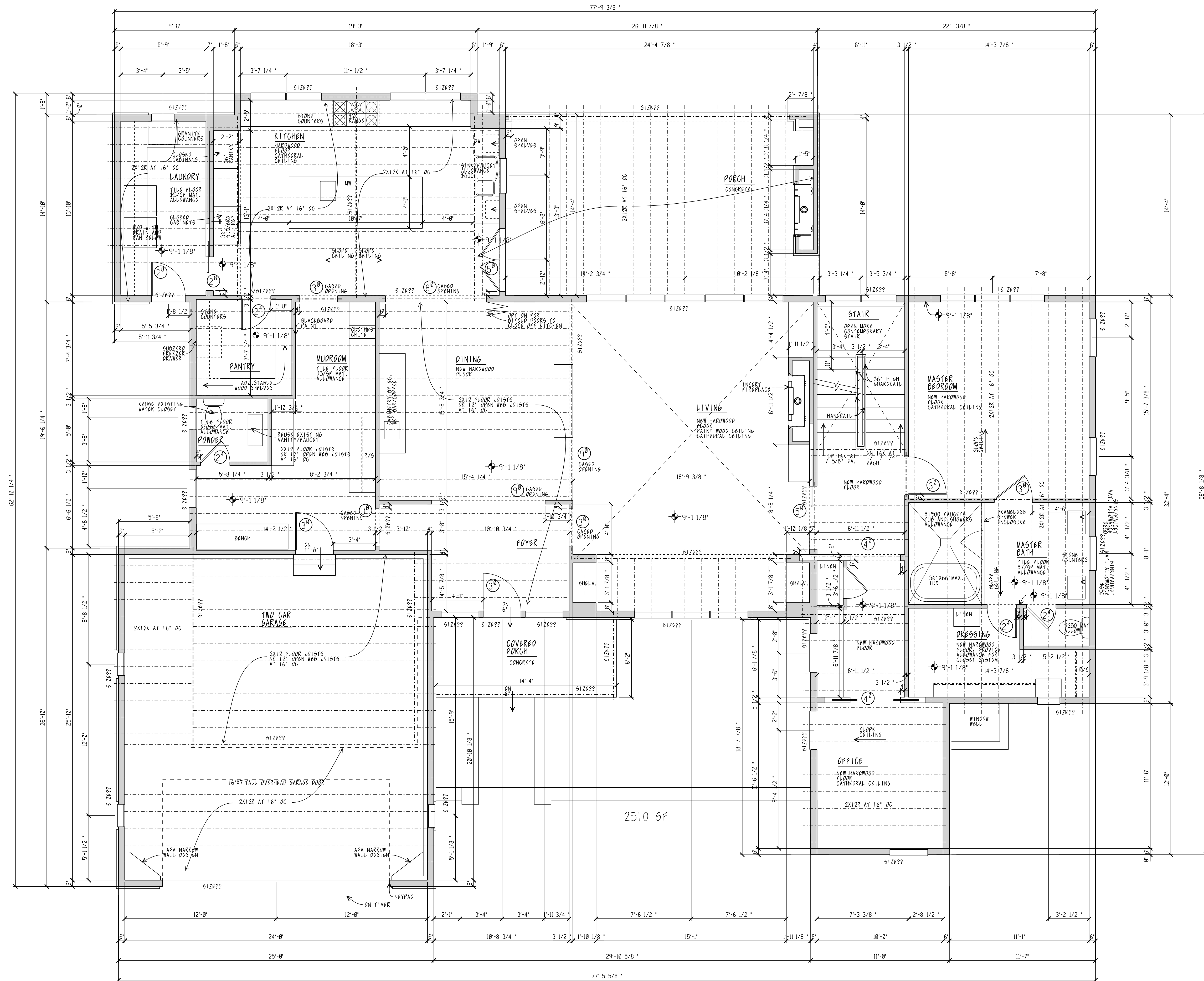
PROPOSED FIRST FLOOR PLAN SCALE: 1/4" = 1'-0"
