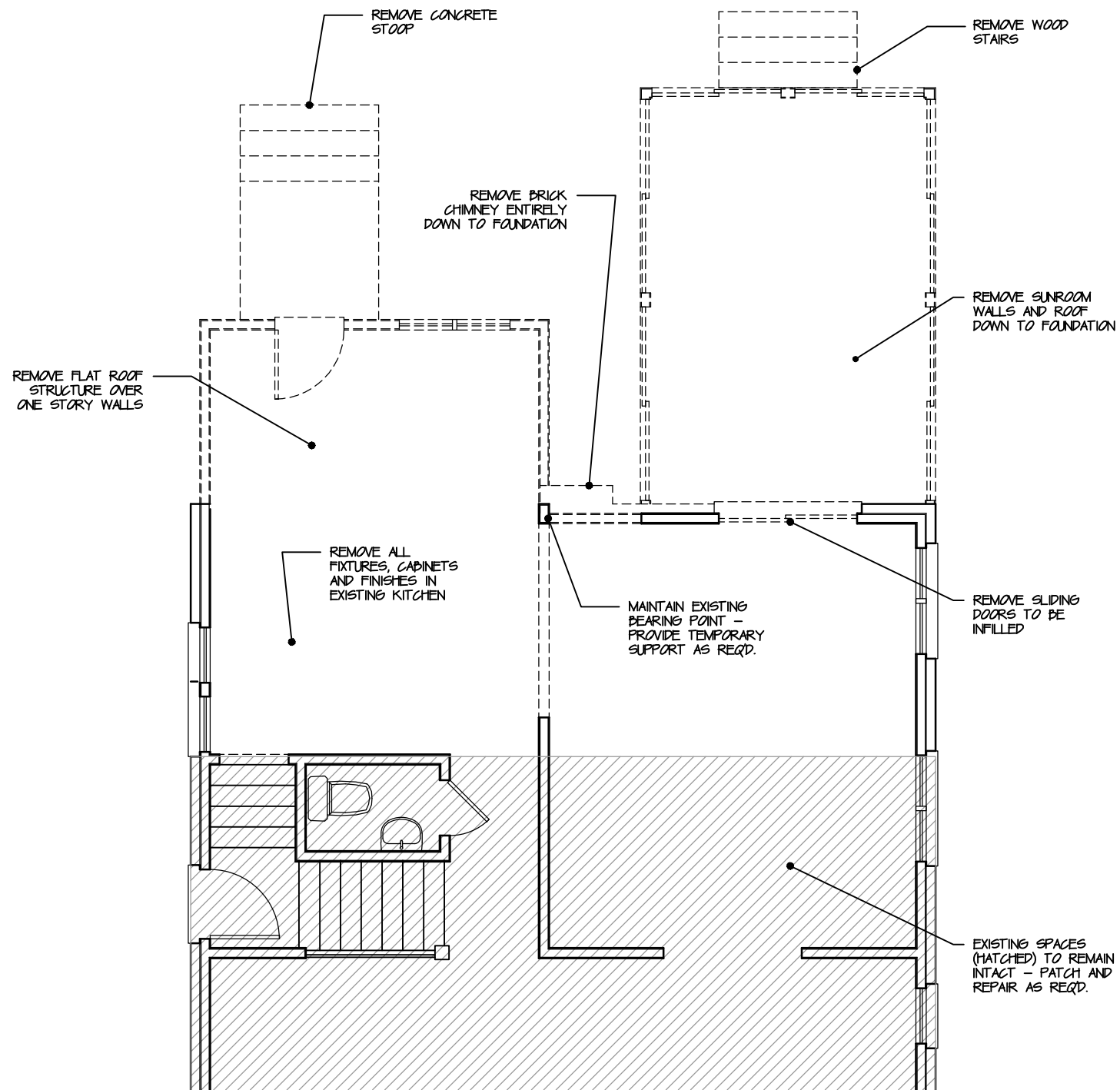
EXISTING/DEMO
