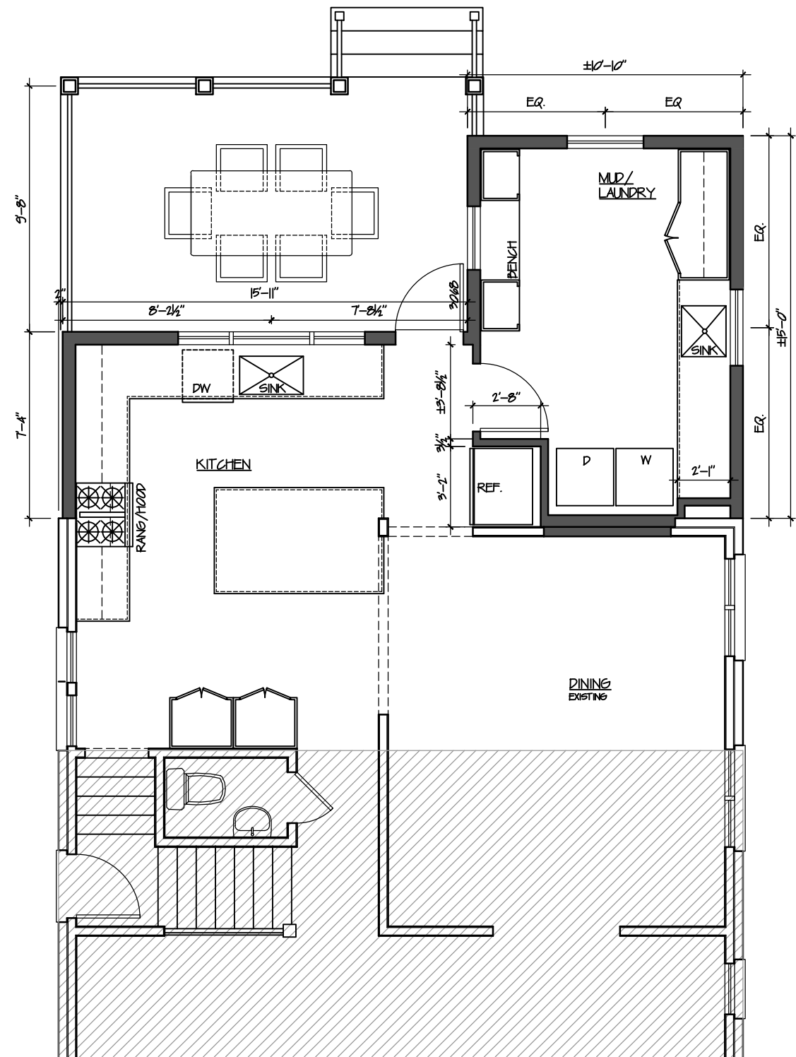
PROPOSED
