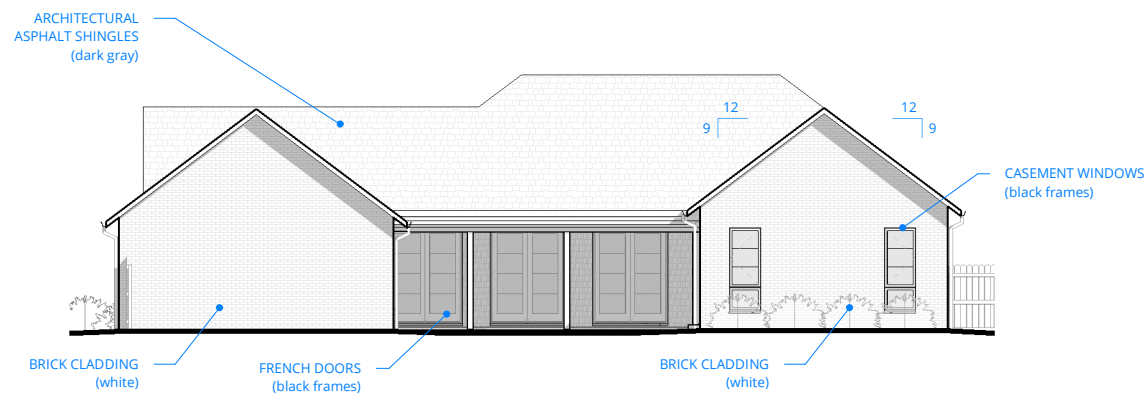
BACK ELEVATION
