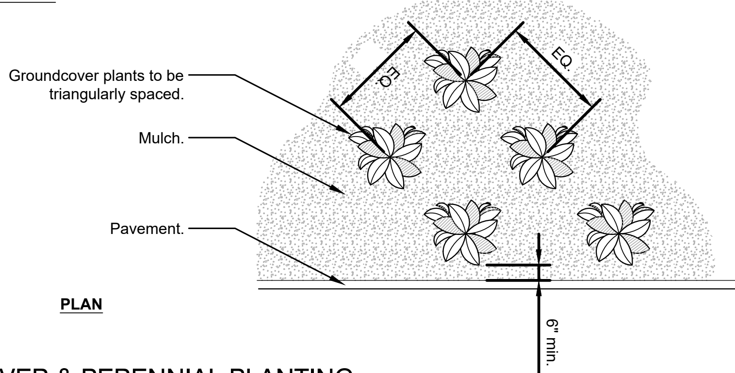
3 GROUNDCOVER & PERENNIAL PLANTING SCALE: 1"=1'-0"
