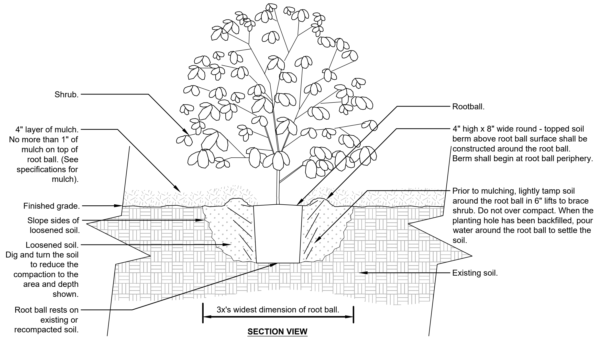
2 SHRUB PLANTING SCALE: 1"=1'-0"
