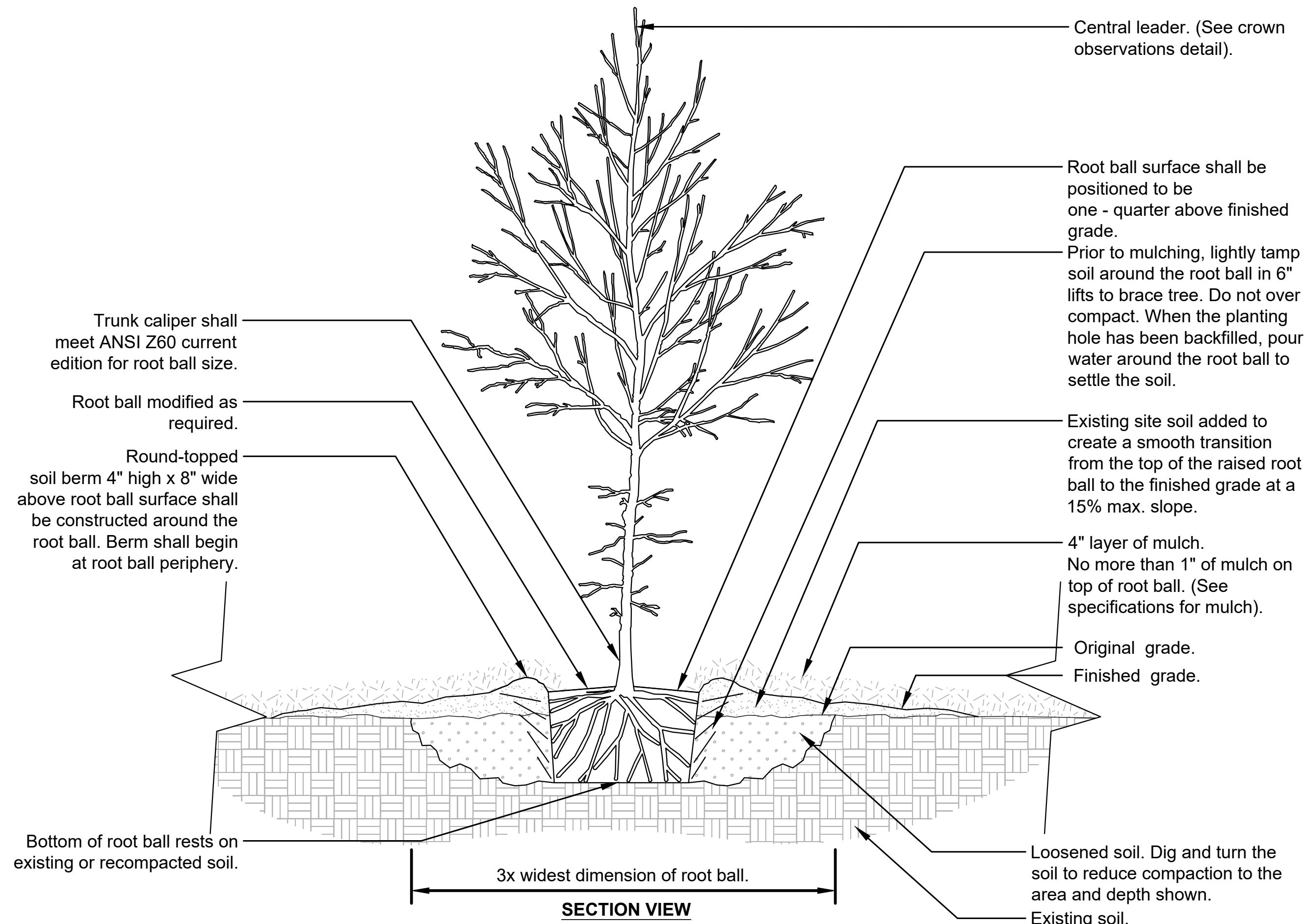
1 TREE PLANTING SCALE: 3/4"=1'-0"
