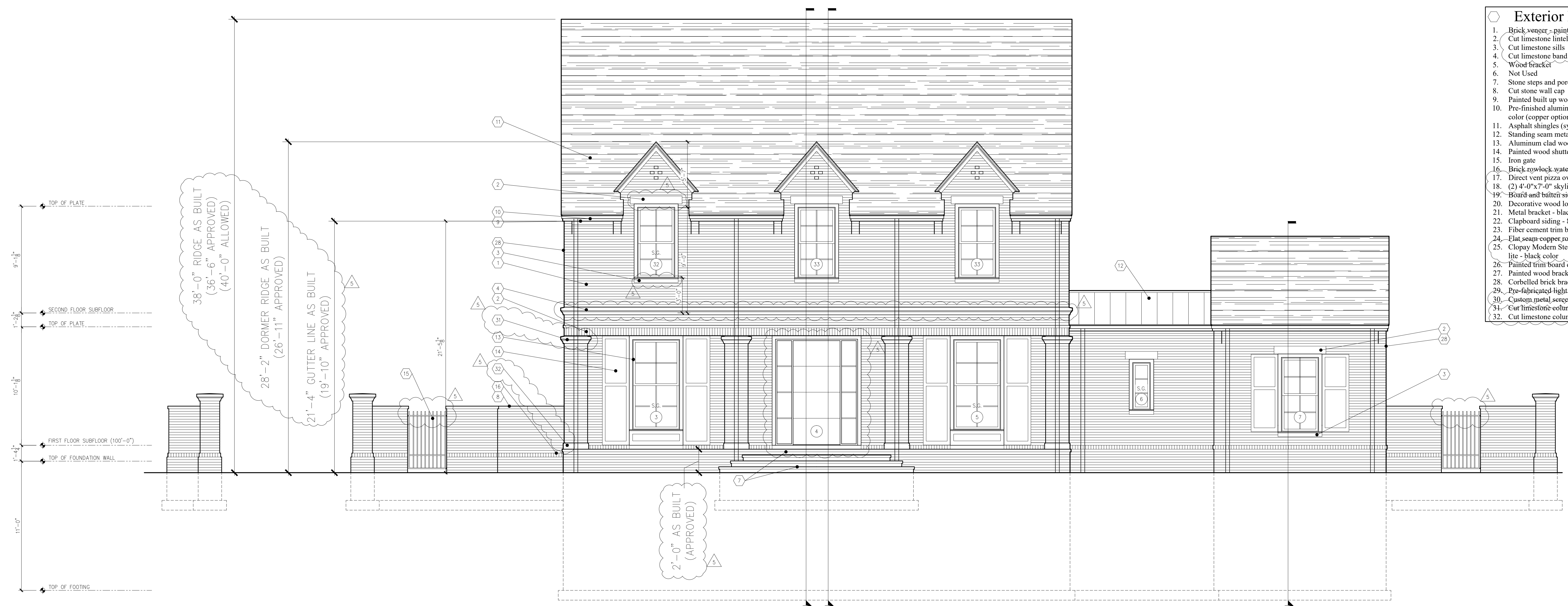
WEST ELEVATION 1/4" = 1'-0"
