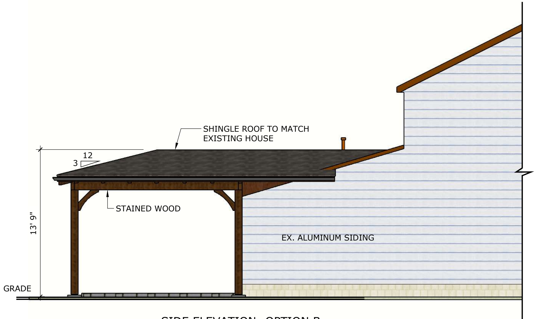
SIDE ELEVATION: OPTION B
