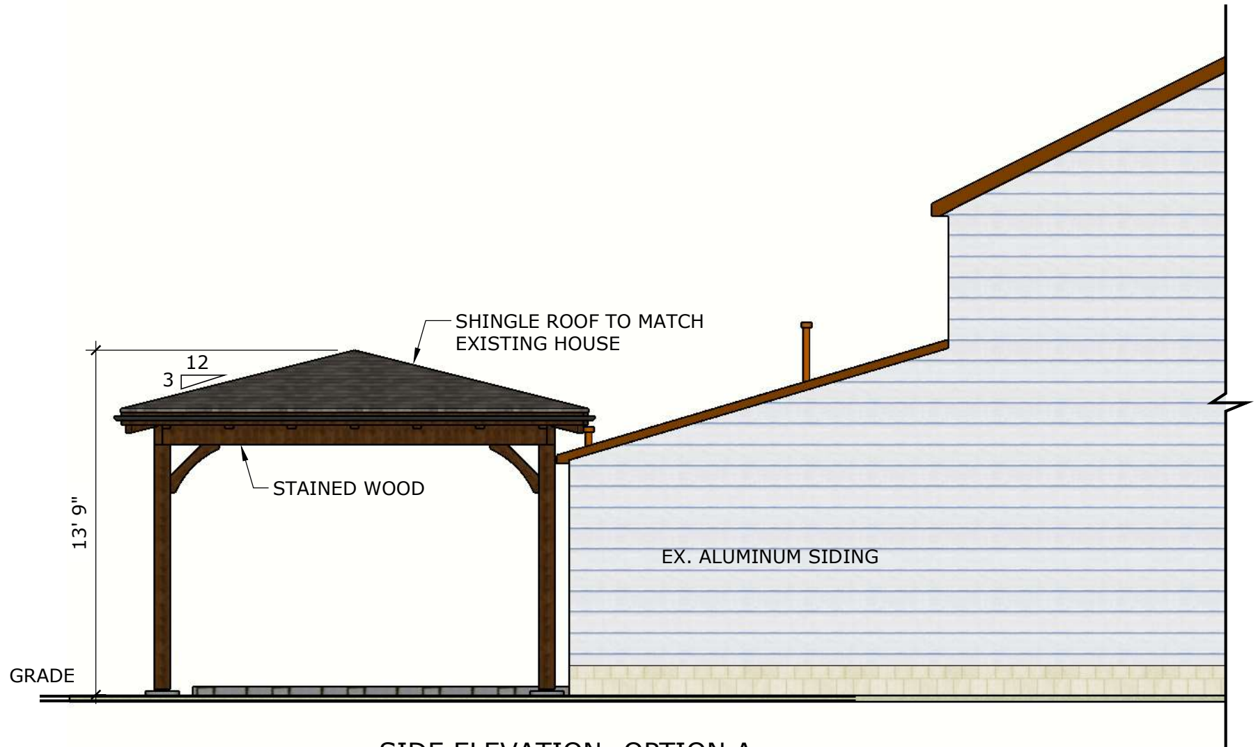
SIDE ELEVATION: OPTION A
