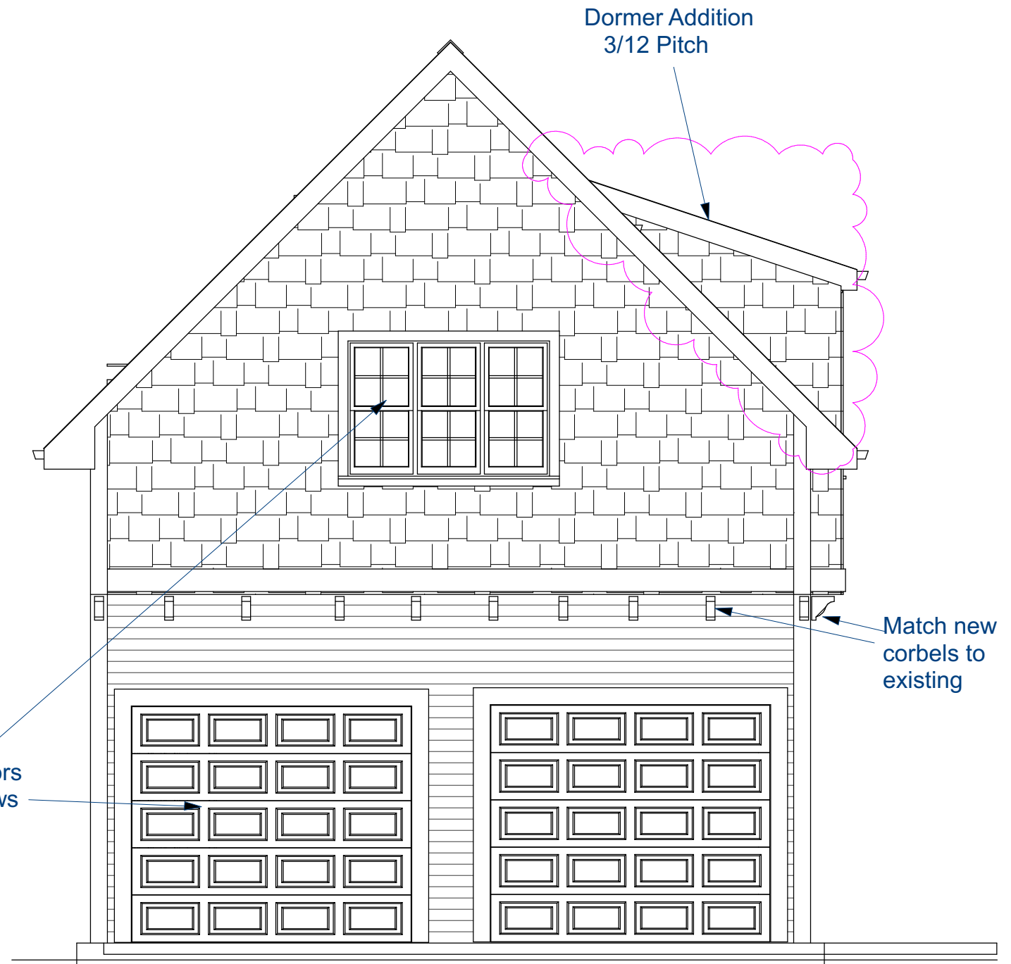
EAST ELEVATION 1/4" = 1'-0"
