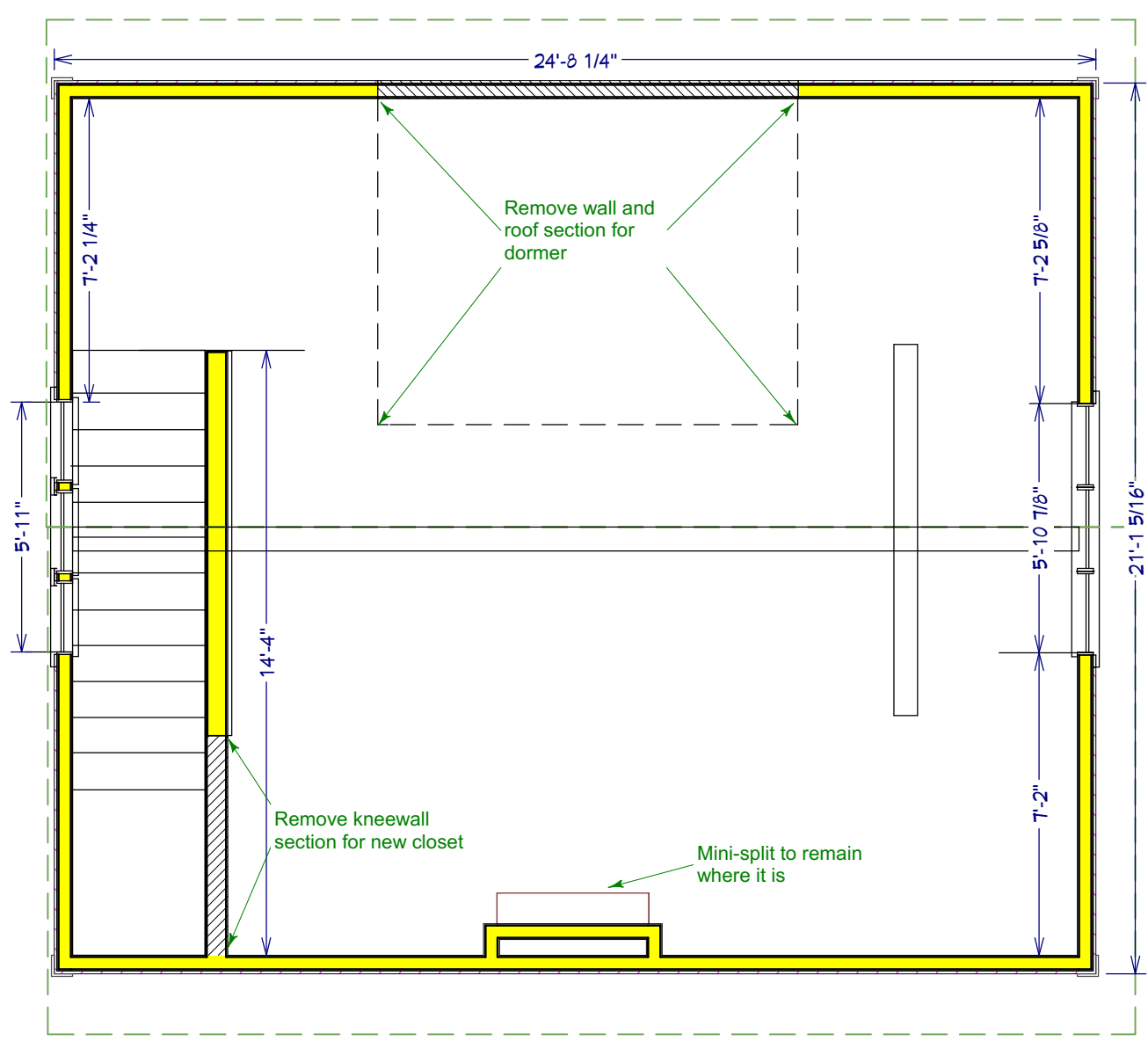
BASS AS-BUILT GARAGE LOFT
