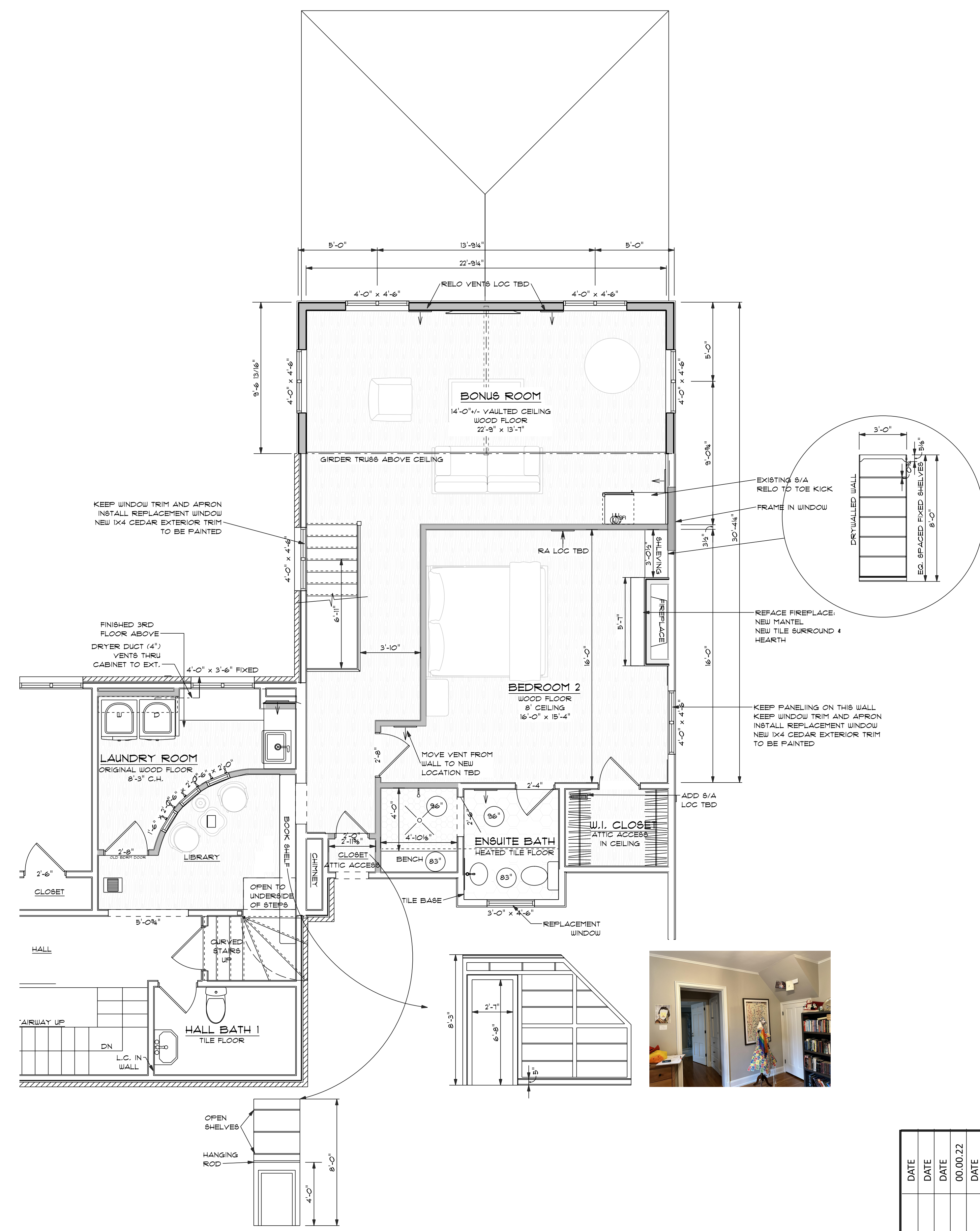
NEW 2ND FLOOR PLAN
