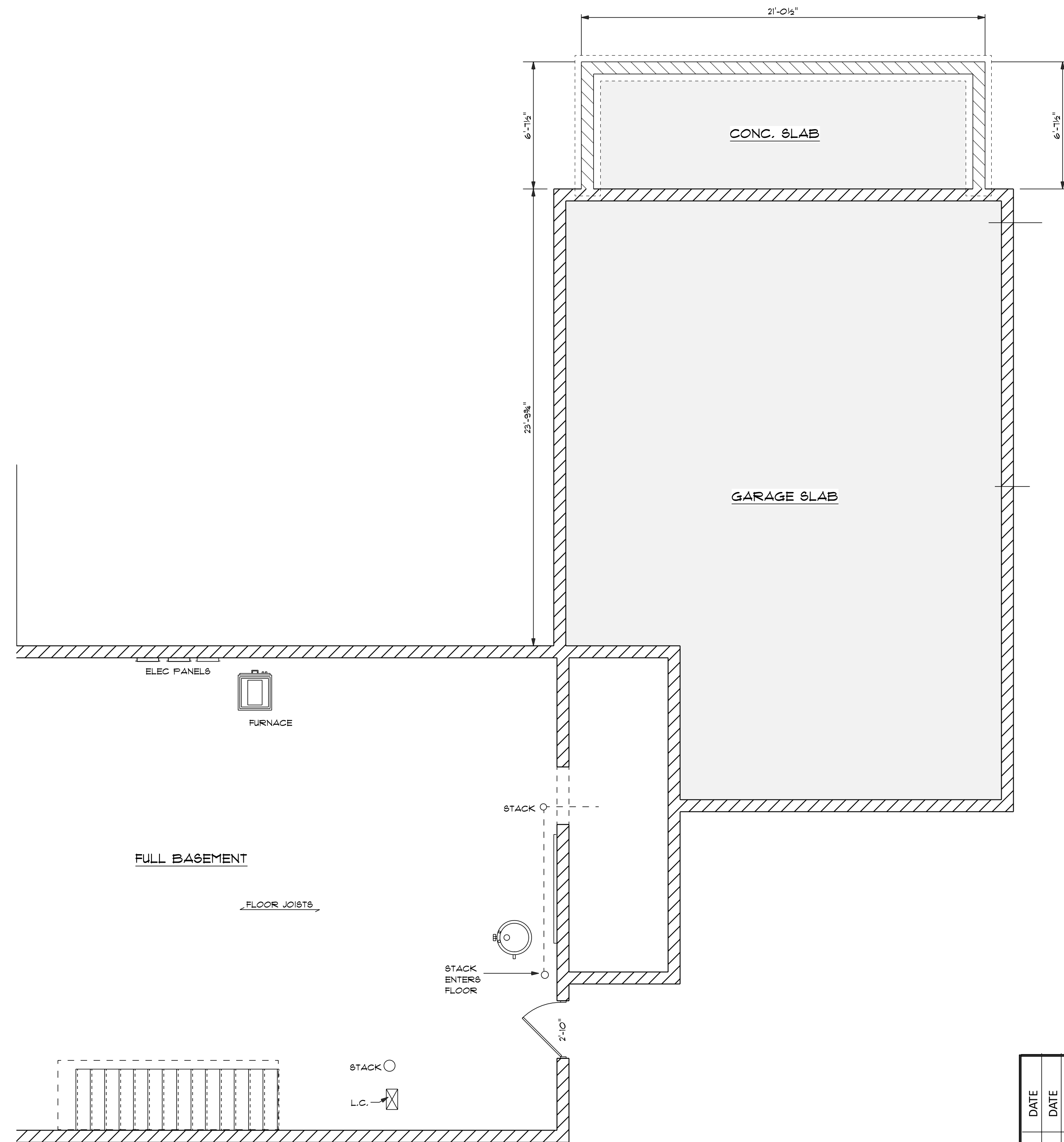
NEW FOUNDATION PLAN
