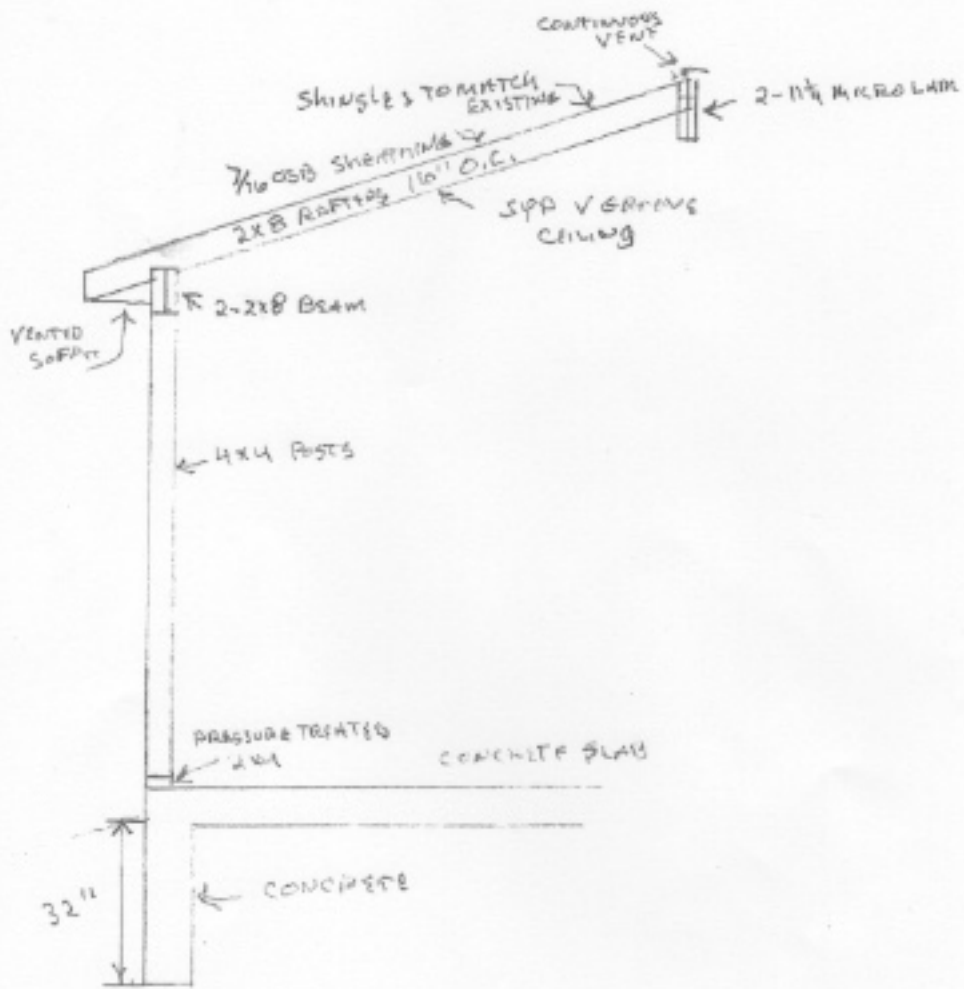
CROSS SECTION
