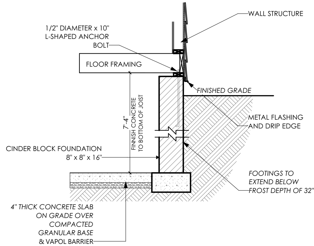
101 FOOTING DETAIL SCALE 1/2"=1'-0"
